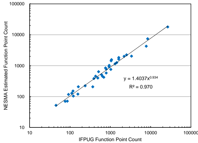
Figure 1. The relationship between IFPUG FP count and NESMA estimated FP (EFP) count.
